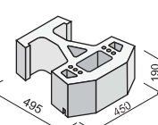
Geostone GWS III. BENT
