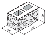
KB 11-21 B RUSTIK
