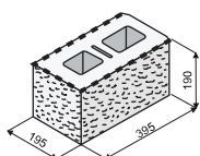
KB 11-21 B
