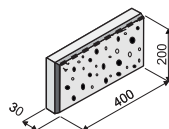
KBF 0-11 G 30
