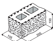
KB 11-21 B GRIND
