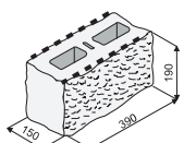
KB 7-15 B GRIND
