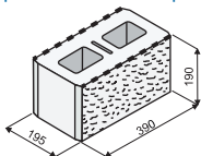
KB 7-21 B
